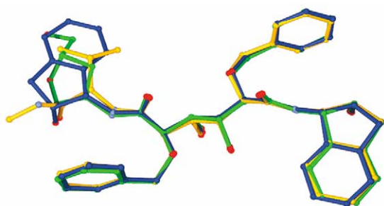
Figure 3. Superimposition of compounds 1a (blue), 1b (gold) and 23 (green) bound to the active site of HIV-1 PR. The image was compiled using Swiss-PDB viewer version 3.51 33 and 3-D-rendered with POV-ray version 3.1. 34
